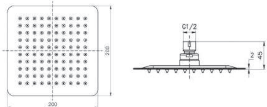
CR - SQ20 - 105
