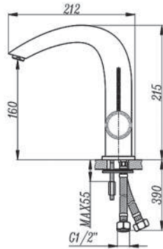
CR - 7362-H24
