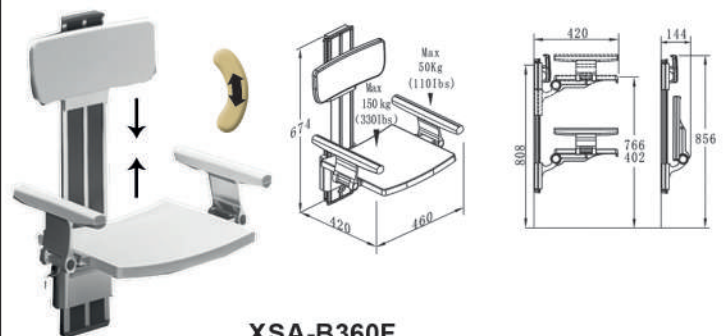
XSA-B360F
